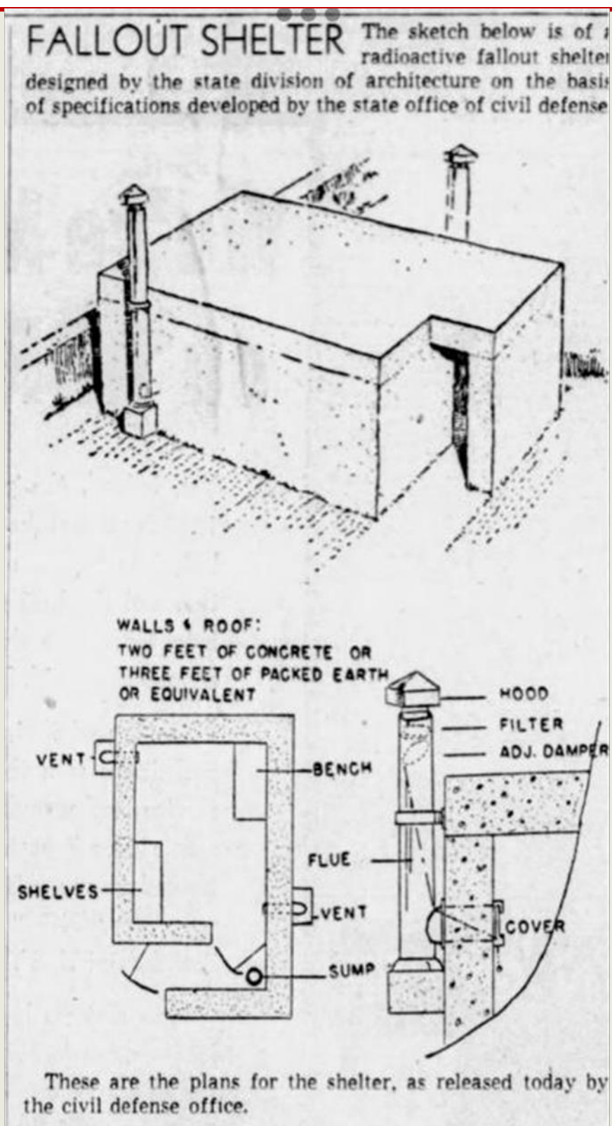
Above are plans for a basic fallout shelter showing the average makeup/layout (Sacramento Bee, March 31, 1955)
